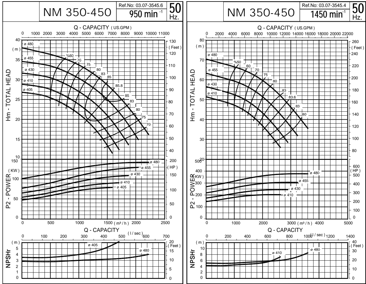
The Performance Curves 50 Hz are based on the kinematic viscosity 1 mm 2 /s and density 1g/cm 3 . Tolerances are acc. to ISO 9906 Annex A.
